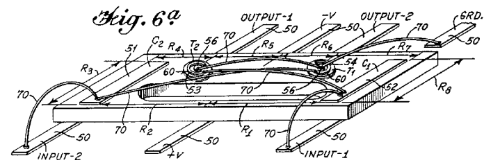
(a) June 23, 1964 J. S. KILBY 3,138,743 MINIATURIZED ELECTRONIC CIRCUITS Filed Feb. 6, 1959 4 Sheets-Sheet 2
